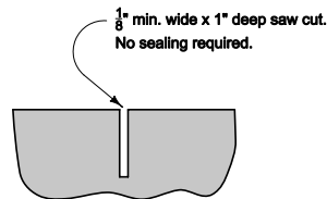
SAWED CONTRACTION JOINT
