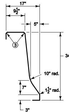
BARRIER FACE
