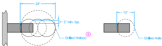
PLAN - CASE A
