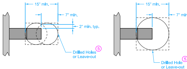
PLAN - PAVEMENT THICKNESS <= 8" Either approach is acceptable.
