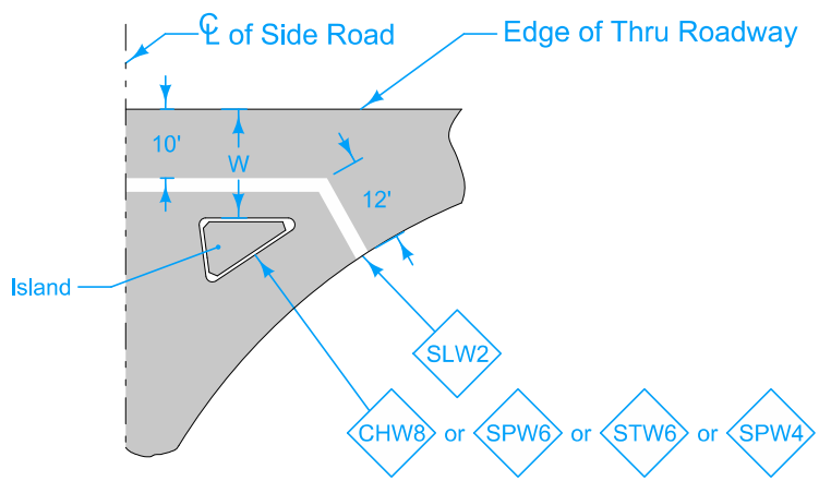
CASE 'C' ISLAND AND W \geq 10 FT.
