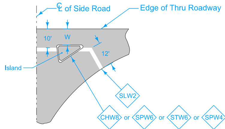
CASE 'B' ISLAND AND W < 10 FT.
