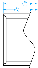
SECTION A-A GROOVE END DETAIL ①
