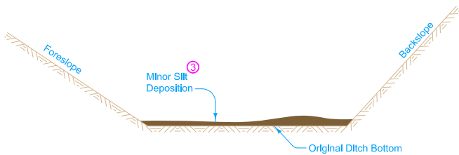
RESHAPING DITCHES
