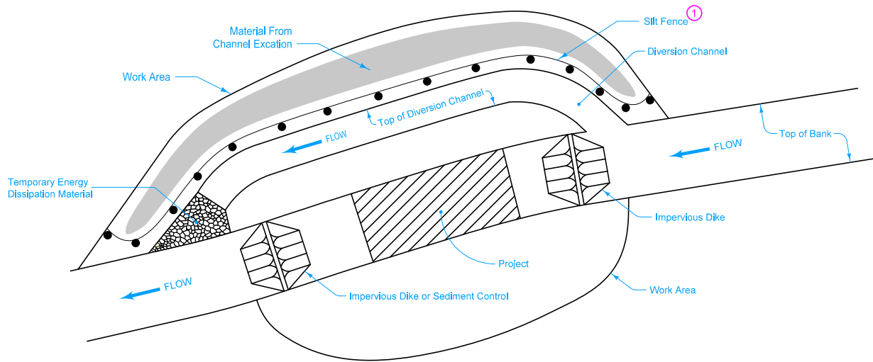
DIVERSION CHANNEL
