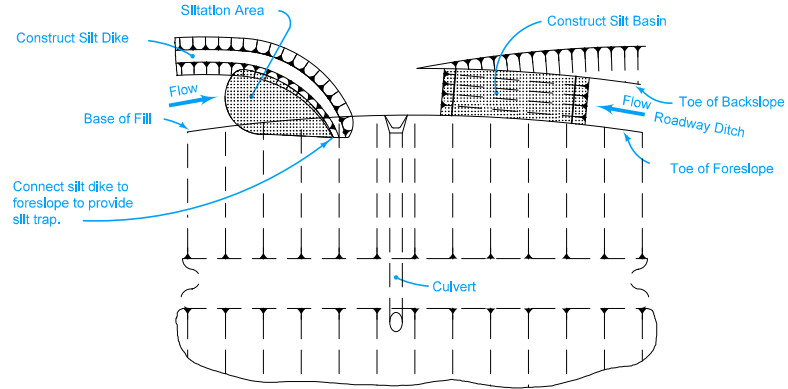
TYPICAL PLAN WITH PERMANENT CULVERT INSTALLATION
